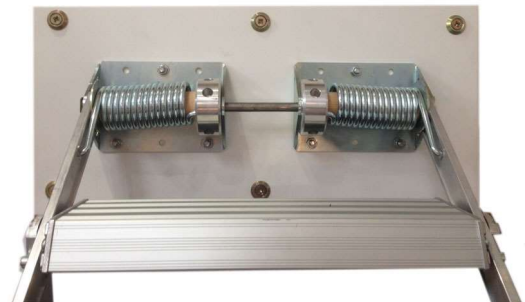
Spring-assisted operation of the retractable ladder (Piccolo Premium)
