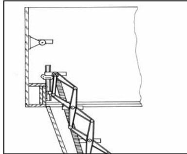
Scheme B: shows two treads fitted above the stairway. A step is formed within the lining and a reduced trapdoor length (110 mm) to create an angle similar to the main stairway.
