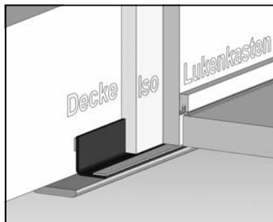
Connection between hatchbox and building (option only for flatroof exits with wooden hatchbox)
